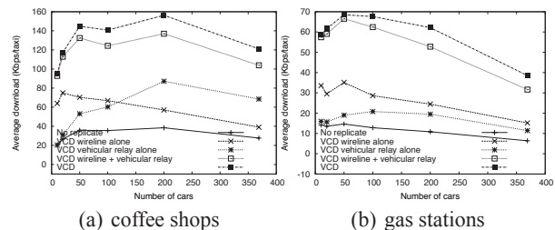
Figure 7: Average throughput under a varying number of vehicles (San Francisco, Zipf-like traffic, range = 100m).
