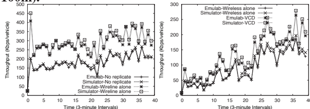
Figure 9: Cross validation: comparing performance in Emulab and simulation
