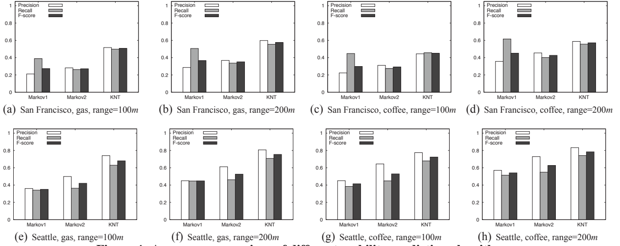
Figure 4: Accuracy comparison of different mobility prediction algorithms.
