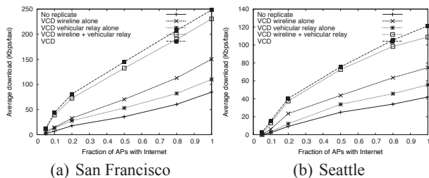
Figure 6: Average throughput under varying fraction of APs with Internet (Zipf-like traffic, APs at coffee shops, range=100, 50 vehicles).
