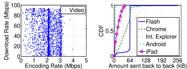
Figure 8: No ON-OFF Cycles. Figure 9: Ack Clock.
