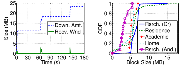
(a) Download Amount and (b) Block Size in the steady state phase.
