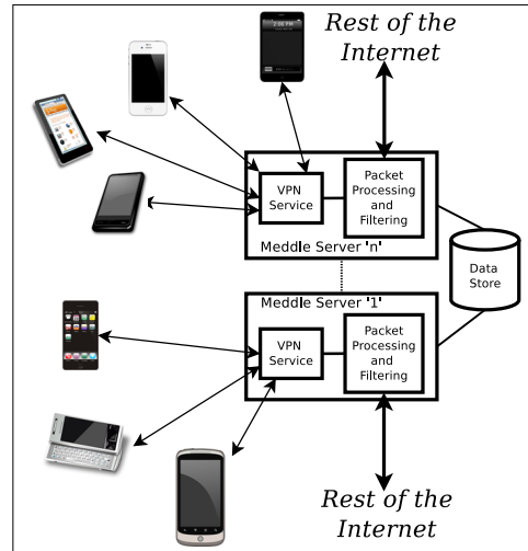
Figure 1: System overview. Clients use VPNs to connect to a nearby Meddle server that interposes traffic.
