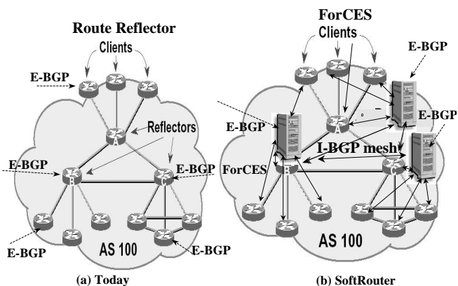
Figure 3: BGP deployment
