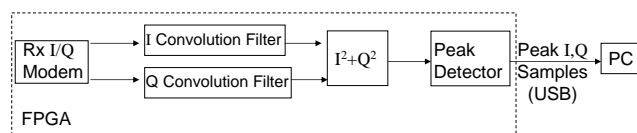
Figure 4: ODS PN-code despreader design.
