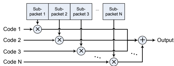
Figure 3: Illustration of bonding. Each sub-packet is spread using a different PN code, and all sub-packets are sent in parallel.
