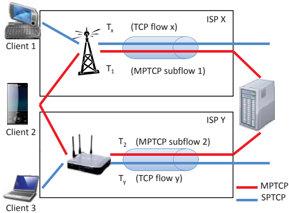
Figure 1: A scenario illustrating competing single-path TCP (SPTCP) and MPTCP connections
