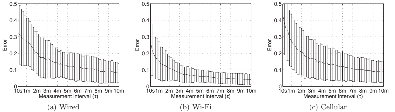
Figure 4: Throughput estimation error for LIA congestion controller
