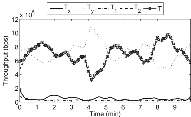
Figure 3: Single-path TCP and MPTCP (OLIA congestion controller) connections compete with each other on paths A and B, which are rate-limited to 1.544 Mbps. Path B is configured with 10 ms delay and 0.01% loss rate, while path A is configured with 250 ms delay and 5% loss rate.
