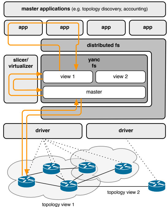
Figure 1: System Architecture
