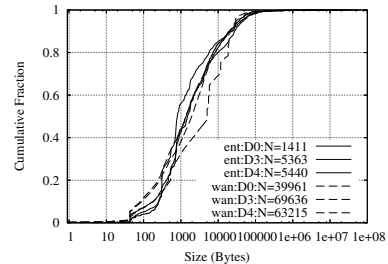
Figure 4: Size of HTTP reply, when present.
