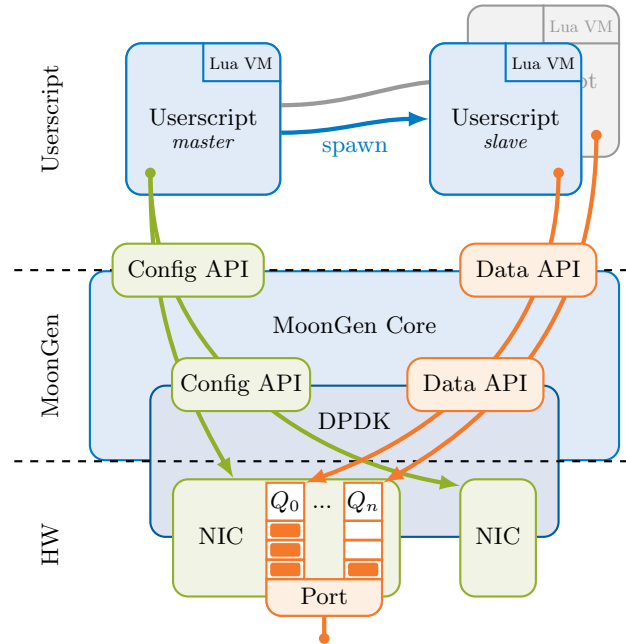
Figure 1: MoonGen’s architecture
