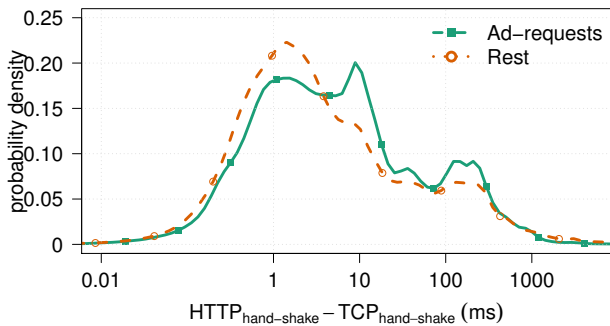
Figure 7: Real time bidding in RBN-2: difference between the HTTP and TCP hand-shake latencies dissected by type of request. The more pronounced modes at 10 ms and 100 ms suggest that ad requests typically involve more back-end functionality than non-ad requests.
