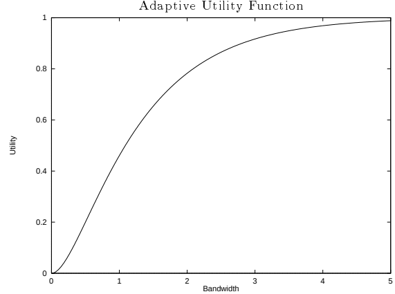
Figure 1: The performance curve \pi(b) for a rate and delay adaptive application.
