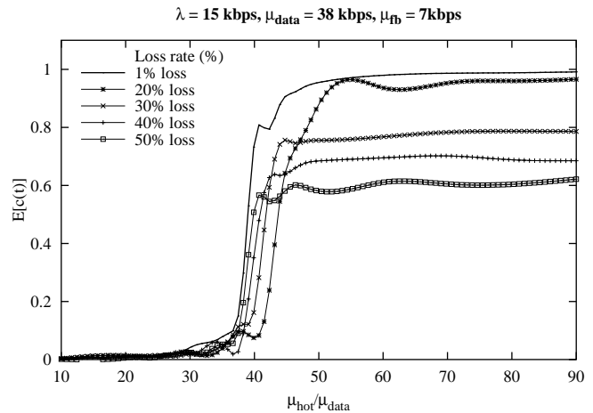
Figure 11: The system consistency shows a “knee”, beyond which the marginal benefit from additional bandwidth to the “hot” queue is limited and below which system consistency shows marked degradation.
