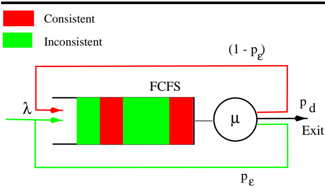
Figure 2: Queuing model for announce/listen-based transport.
