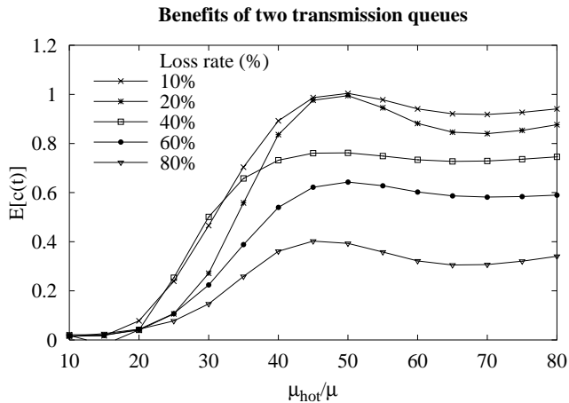
Figure 5: Two-level scheduling improves consistency by 10% to 40%. \mu_{data} = 45kbps , \lambda = 15kbps . Consistency is maximum when \mu_{hot} > \lambda .
