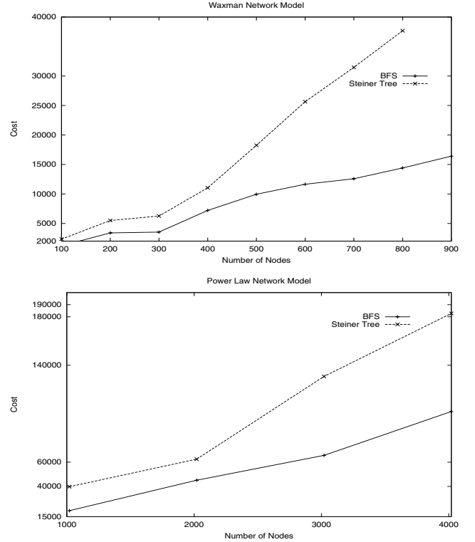
Figure 7: Effect of Number of Network Nodes on Performance of Algorithms.
