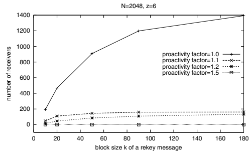
Figure 16: Expected number of receivers satisfying C0
