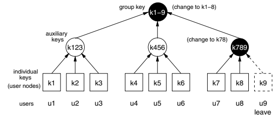
Figure 2: An example key tree
