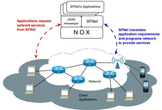
Figure 2: Architecture of SFNet
