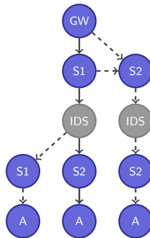
Figure 5: Example forwarding graph.
