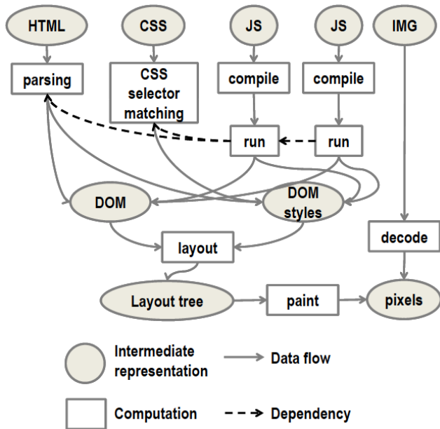
Figure 3: Data flow of processing an example Web page. Note that some IRs for evaluating JavaScript are omitted here.
