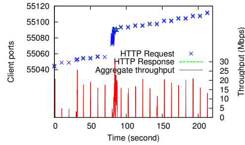
Figure 24: The periodic request behavior of Netflix player limiting its overall throughput.
