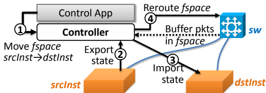
Figure 1: Parts of an NF state management framework, and the steps for a move operation; packet buffering is required for loss-free moves
