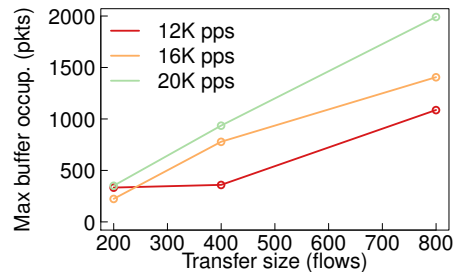
Figure 2: Required buffer capacity when moving state for n flows with a traffic rate of r pps
