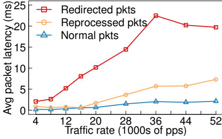
Figure 4: Improvements in latency overhead
