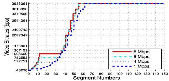
Figure 2: Bitrate Access Patterns for DASH video
