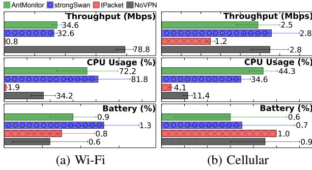
Figure 2: Performance of AntMonitor, strongSwan, tPacket-Capture, and NoVpn when downloading 1 GB file on Wi-Fi 802.11ac and 100 MB file on 4G LTE.
