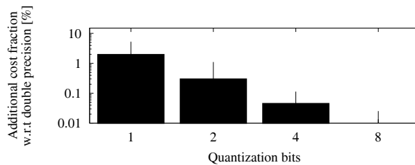
Figure 7: Robustness against implementation constraints: while price quantization affects accuracy of the decisions, the net effect is a negligible cost increase for the ISP.
