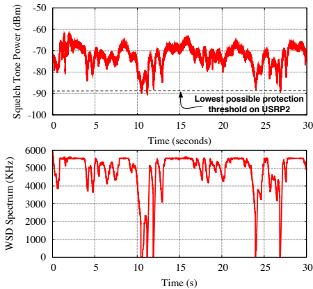
Figure 23: Robustness to avoid disruption, adapting the channel.
