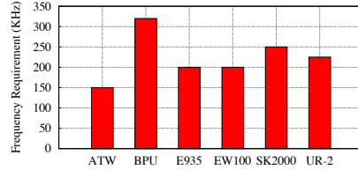
Figure 8: The frequency tolerance thresholds for all of the mics for no audible interference.
