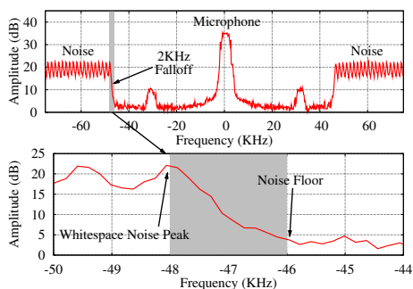
Figure 12: Illustrating the falloff to reach the noise floor in 2KHz.
