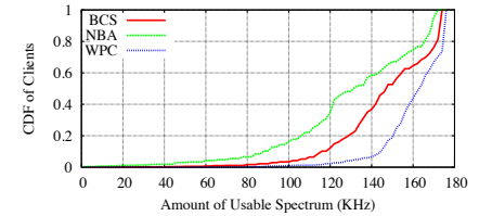
Figure 26: CDF of available spectrum.
