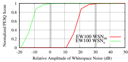
Figure 4: Audible interference, varying WSN. Areas where score reaches 1 are highlighted.
