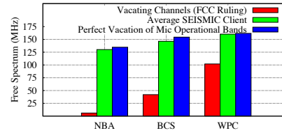
Figure 25: Comparing available spectrum.
