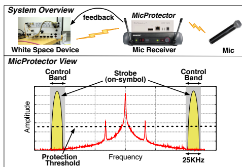
Figure 13: Overview of SEISMIC and MicProtector.
