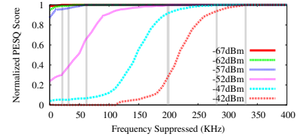
Figure 9: Varying WSD interf. power at mic receiver, suppression needed varies greatly.
