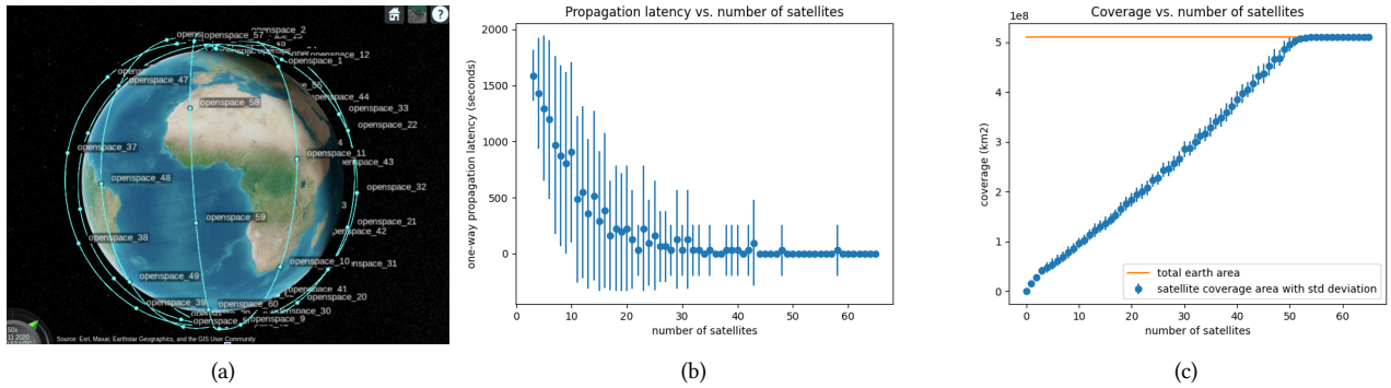
Figure 2: (a) A simulated OpenSpace constellation. This configuration achieves global coverage while maintaining inter-satellite distances and trajectories that allow for simple and sustained ISLs. (b) Propagation latency achieved by an increasing number of satellites in a constellation. From the latency results, the constellation requires a minimum of about four satellites to guarantee that a satellite will orbit in range of the user’s or ground station’s location. (c) Coverage achieved by an increasing number of satellites in a constellation. Additional satellites above the minimum for total earth coverage ensure fault tolerance, increased throughput and bandwidth capabilities, and increased availability in regions with signal-attenuating landscapes.
