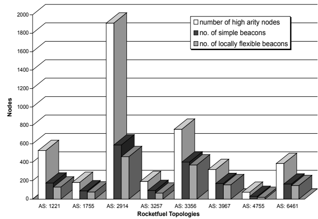
Figure 4: Histogram of beacon set sizes yielded by different algorithms for the Rocketfuel topologies.
