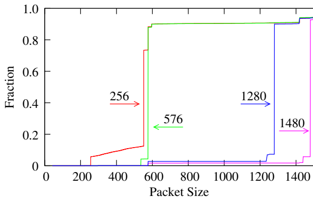
Figure 5: The subsequent size of a segment after a PTB message is sent, for each MTU tested. Most webservers behave as expected and reduce their packet size to the size advised, although most webservers will not reduce their packet size below 552 bytes if asked.
