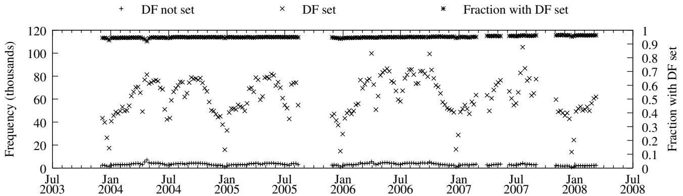
Figure 1: IPv4 webservers that send data packets with the DF bit set over time as measured by packet traces at the edge of the University of Waikato network. Each point represents one week. The bottom series is the number of webservers that never set the DF bit on any data packet. The middle series is the number of webservers that set the DF bit on all data packets. The top series is the fraction of these webservers that always set the DF bit; the fraction grows from 94% in 2004 to 96% by 2008.
