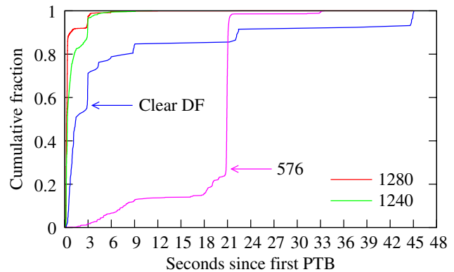
Figure 6: The delay between the first PTB sent and the action by the host. The delays measured in reducing to 576 bytes suggest the reductions are due to the hosts filtering PTB messages but having PMTUD blackhole detection enabled.
