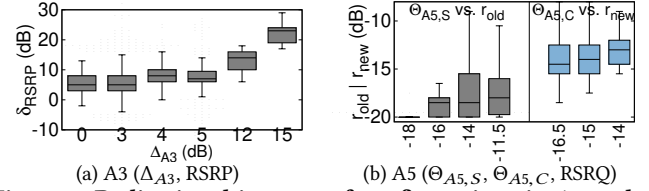
(a) A3 ( \Delta_{A3} , RSRP) (b) A5 ( \Theta_{A5,S} , \Theta_{A5,C} , RSRQ) Figure 9: Radio signal impacts of configurations in A3 and A5.
