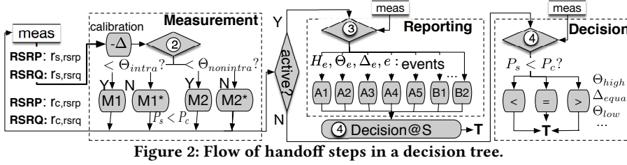
Figure 2: Flow of handoff steps in a decision tree.
