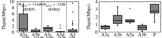
(a) Impact on throughput (AT&T) (b) Impact on throughput (T-Mobile) Figure 8: Impacts of reporting event configurations.
