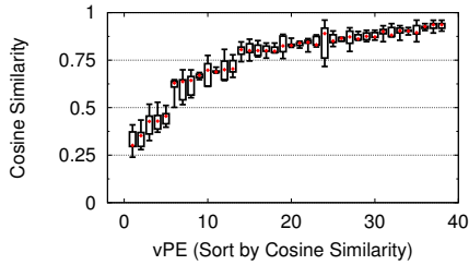
Figure 3: Cosine similarity of syslog distribution between all vPEs and individual vPE.
