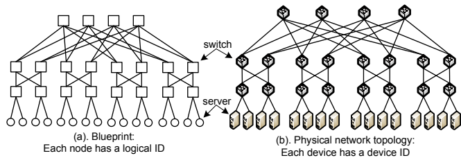
Figure 1: An example of blueprint, and physical topology constructed by following the interconnections in blueprint.
