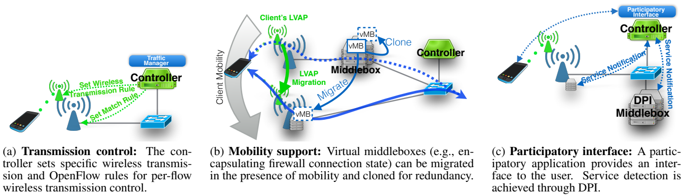
Figure 1: Three basic operations supported by OPENSOWN.
