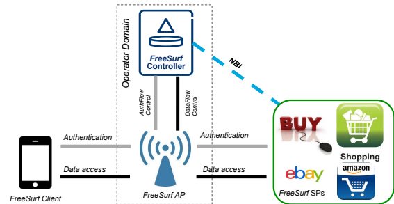
Figure 1: FreeSurf overview.
