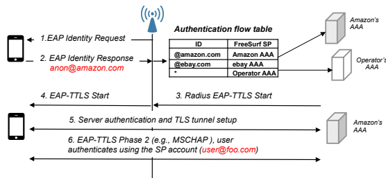
Figure 2: FreeSurf authentication.
