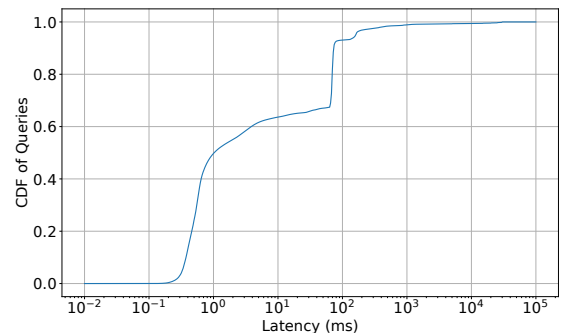
Figure 12: CDF of user DNS query latencies seen at a recursive resolver at ISI, over the course of one year. Latencies are measured from the timestamp when the recursive resolver receives a client query to the timestamp when the recursive sends a response to that client query. The sub-millisecond latency for more than half of queries suggests most queries to this recursive are served by the local cache.
