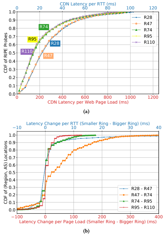
Figure 4: RTTs and latencies per web page load from RIPE probes to CDN rings (4a), and change in median latency for Microsoft users in \langle region, AS \rangle locations when transitioning rings (4b). Axes with per-RTT latencies are blue, while axes with per-page-load latencies are red. Latencies per page load can be significant, so Microsoft has an incentive to reduce inflation.
