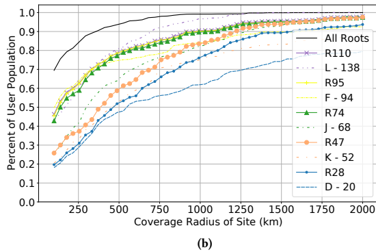
Figure 7: Larger deployments lead to lower latency (Fig. 7a-left) since they offer more low-latency options to users (Fig. 7b). However, fewer users visit their closest site (Fig. 7a-right) leading to more inflation.
