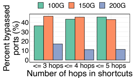
Figure 11: Modulation formats on shortcuts of different lengths. As the number of shortcut hops increases, the fraction of ports in higher modulation formats reduce.
