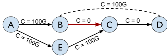
Figure 16: Tunnel AECD is removed when wavelengths of edges BC and CD are allocated to shortcut BD. Nodes B and C can no longer communicate in the bypass-enabled network.
