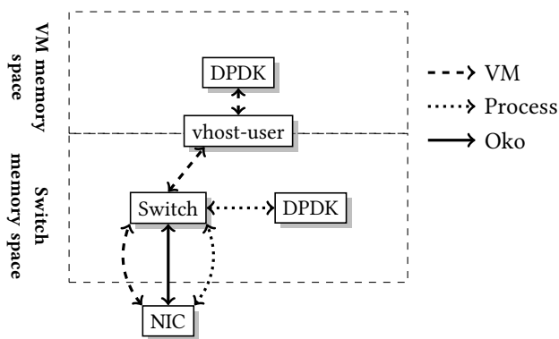
Figure 7: The three evaluation setups for the end-to-end performance comparison. Packet copies are only necessary when crossing memory space boundaries.
